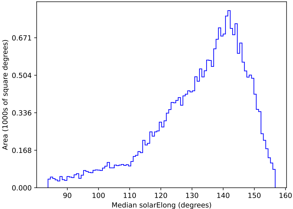
too_elab_r8_d3_giz_v3.4_10yrs All sky g band: Median solarElong
