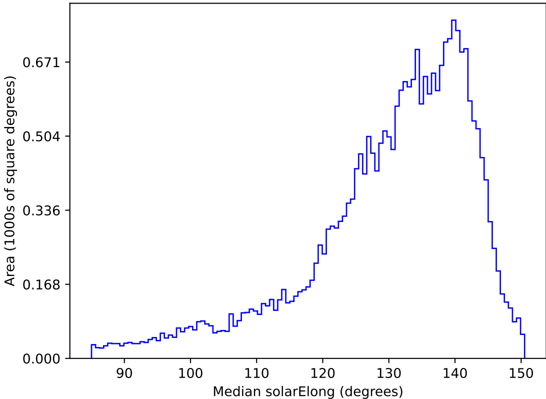
too_elab_r8_d3_giz_v3.4_10yrs All sky all bands: Median solarElong
