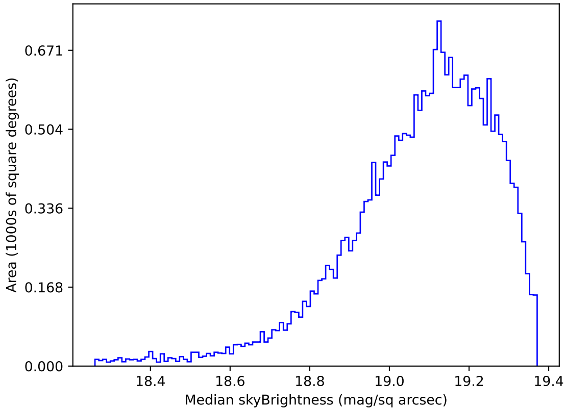
too_elab_r8_d3_giz_v3.4_10yrs Yr 1 z band: Median skyBrightness
