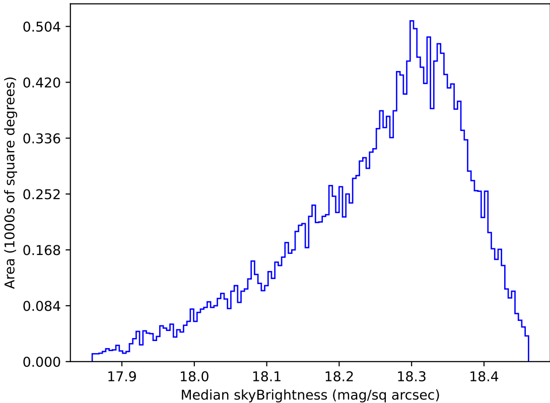
too_elab_r8_d3_giz_v3.4_10yrs Yr 1 y band: Median skyBrightness
