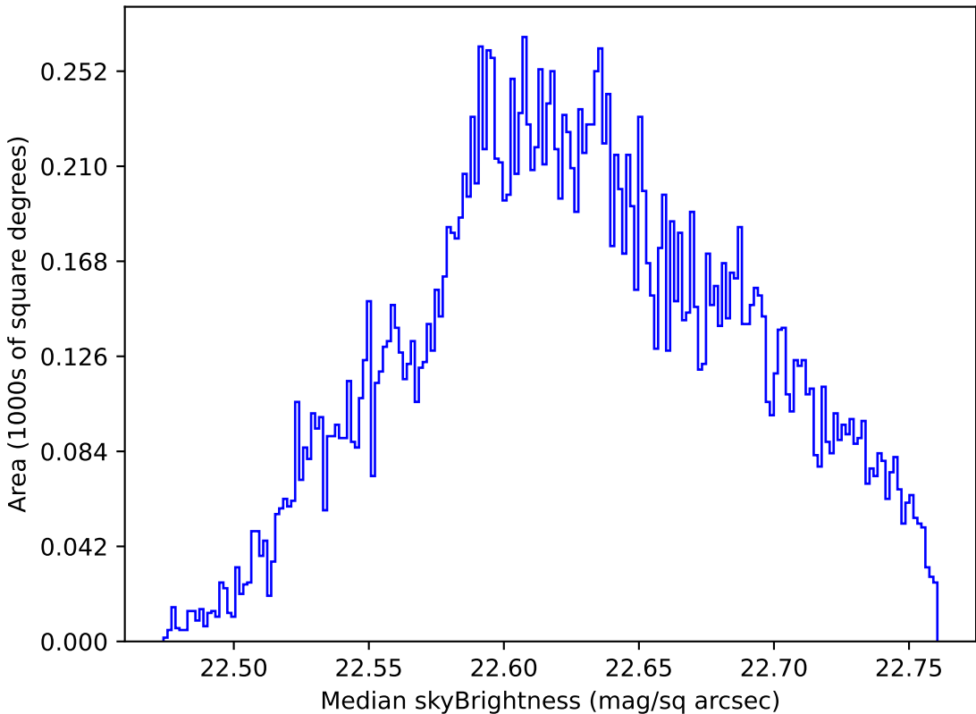
too_elab_r8_d3_giz_v3.4_10yrs Yr 1 u band: Median skyBrightness
