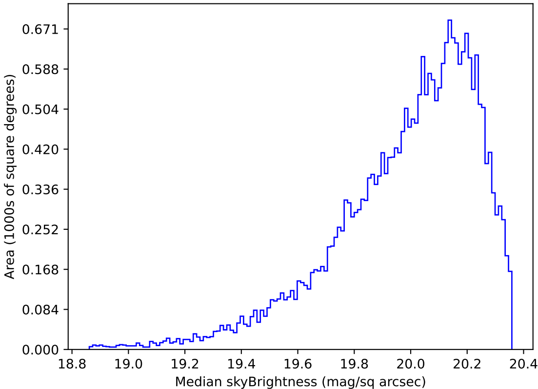
too_elab_r8_d3_giz_v3.4_10yrs Yr 1 i band: Median skyBrightness
