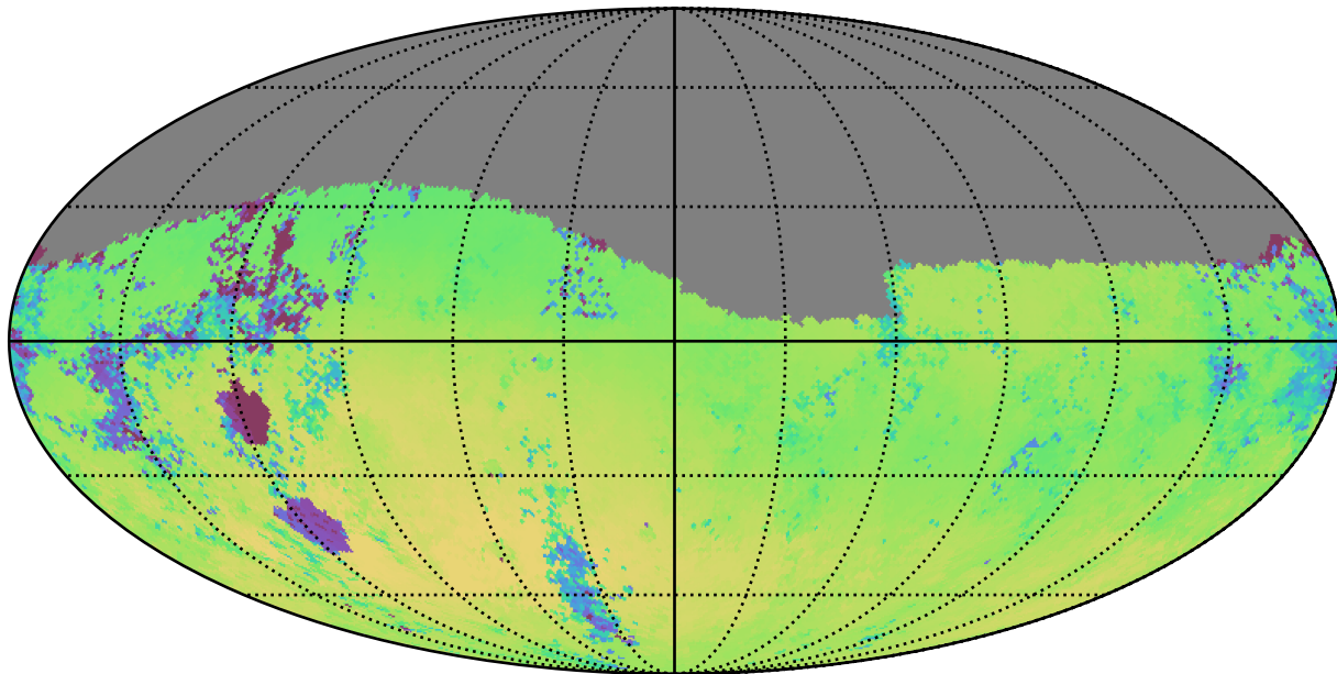
too_elab_r8_d3_giz_v3.4_10yrs Yr 1 g band: Median skyBrightness
