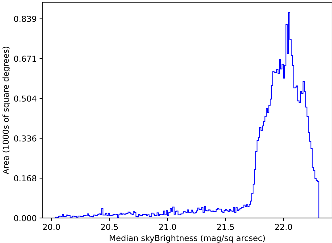
too_elab_r8_d3_giz_v3.4_10yrs Yr 1 g band: Median skyBrightness
