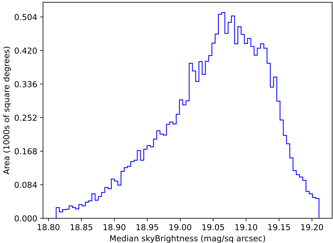
too_elab_r8_d3_giz_v3.4_10yrs WFD z band: Median skyBrightness
