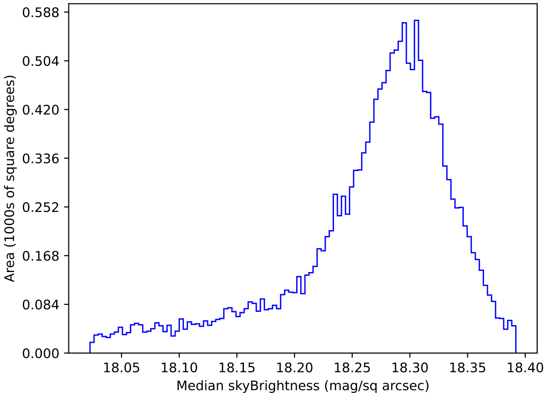
too_elab_r8_d3_giz_v3.4_10yrs WFD y band: Median skyBrightness
