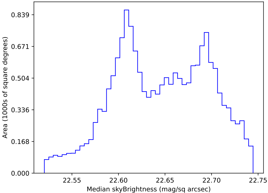
too_elab_r8_d3_giz_v3.4_10yrs WFD u band: Median skyBrightness
