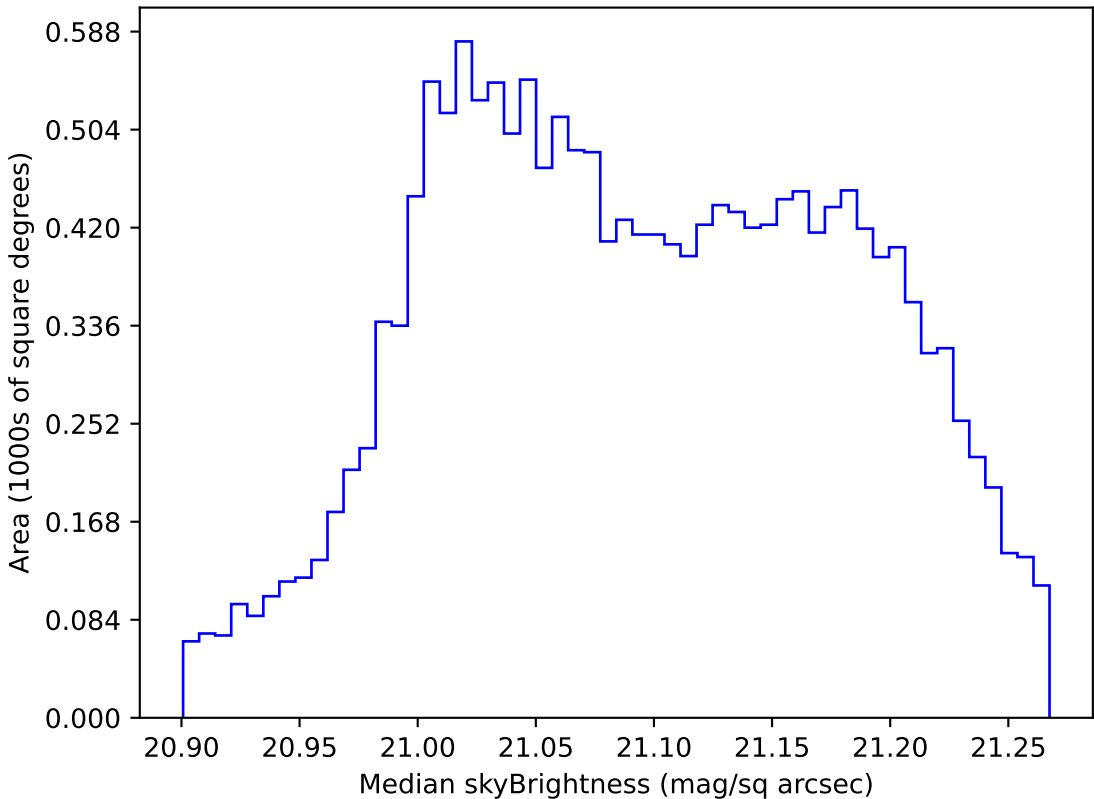
too_elab_r8_d3_giz_v3.4_10yrs WFD r band: Median skyBrightness
