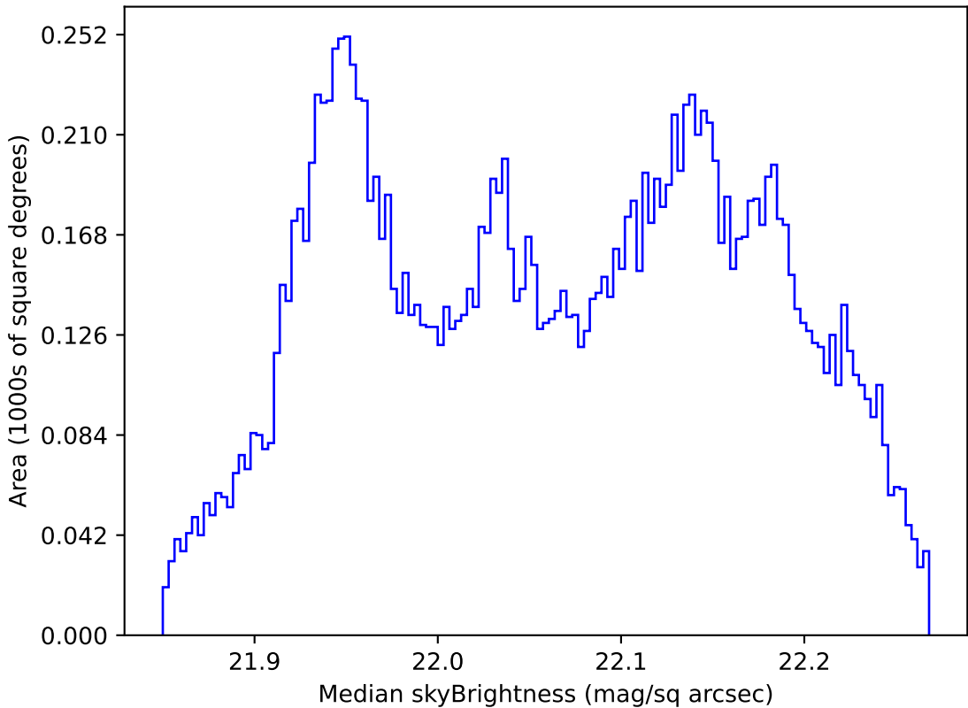
too_elab_r8_d3_giz_v3.4_10yrs WFD g band: Median skyBrightness
