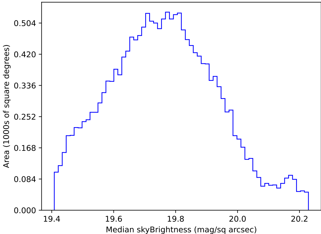
too_elab_r8_d3_giz_v3.4_10yrs WFD all bands: Median skyBrightness
