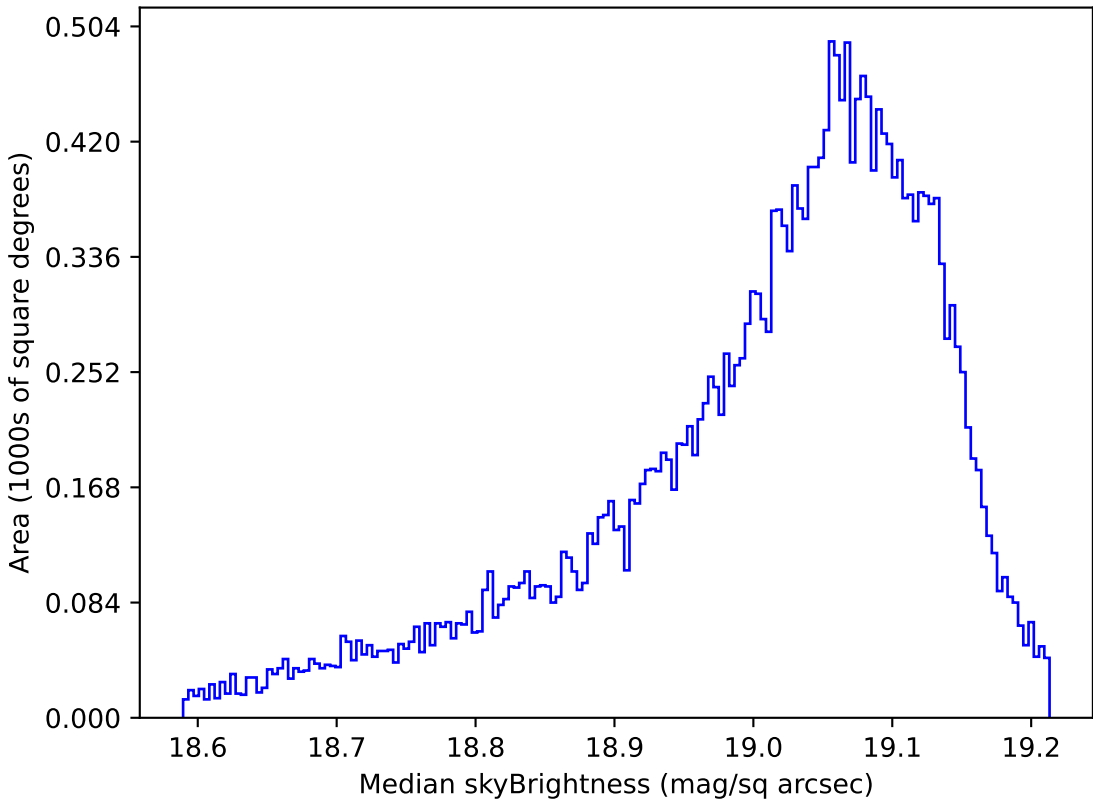
too_elab_r8_d3_giz_v3.4_10yrs All sky z band: Median skyBrightness
