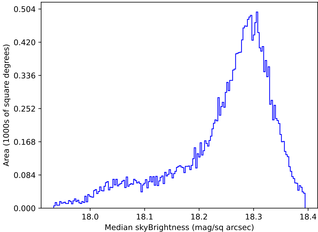
too_elab_r8_d3_giz_v3.4_10yrs All sky y band: Median skyBrightness
