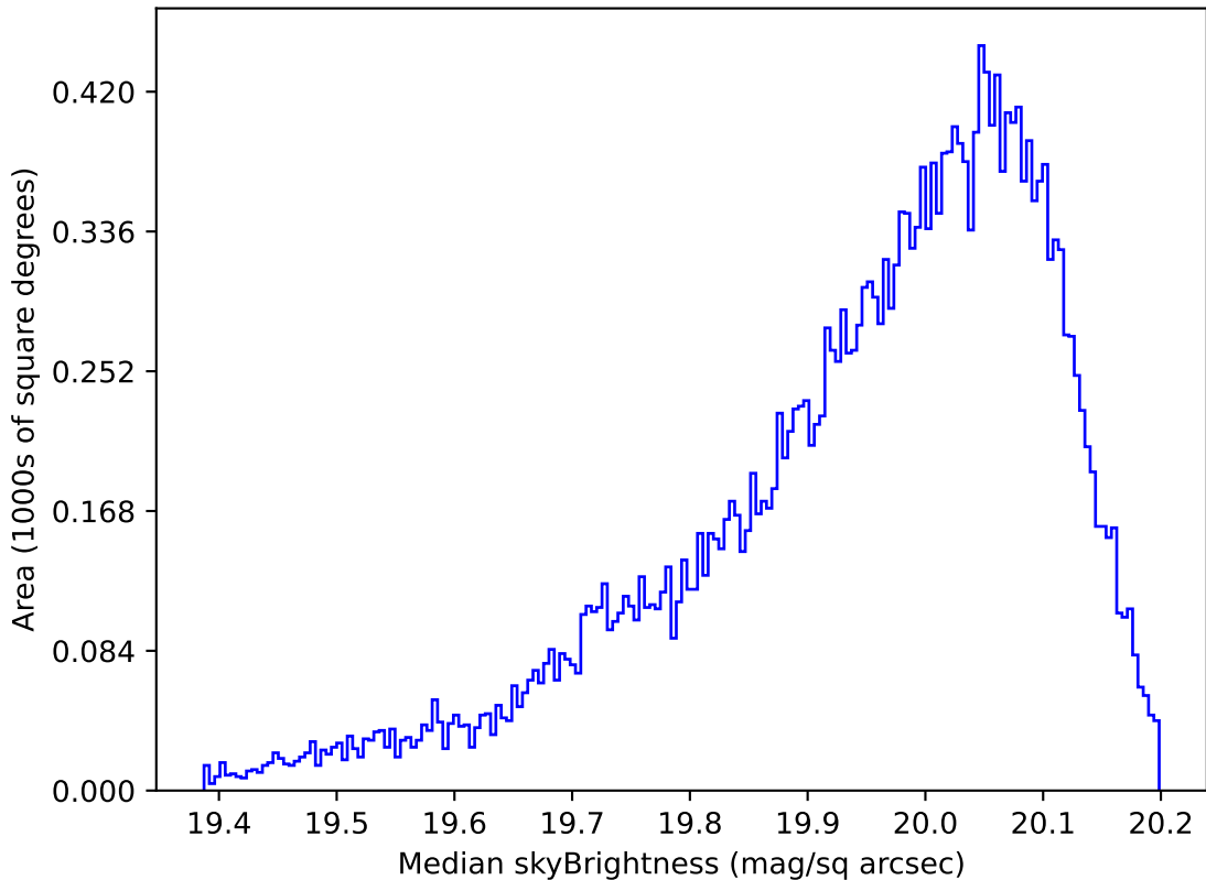
too_elab_r8_d3_giz_v3.4_10yrs All sky i band: Median skyBrightness
