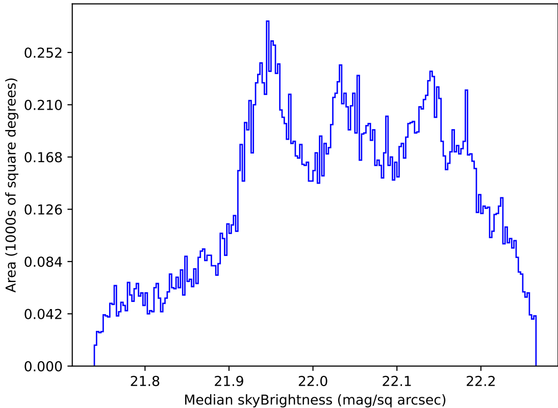
too_elab_r8_d3_giz_v3.4_10yrs All sky g band: Median skyBrightness
