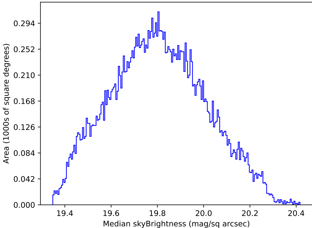
too_elab_r8_d3_giz_v3.4_10yrs All sky all bands: Median skyBrightness
