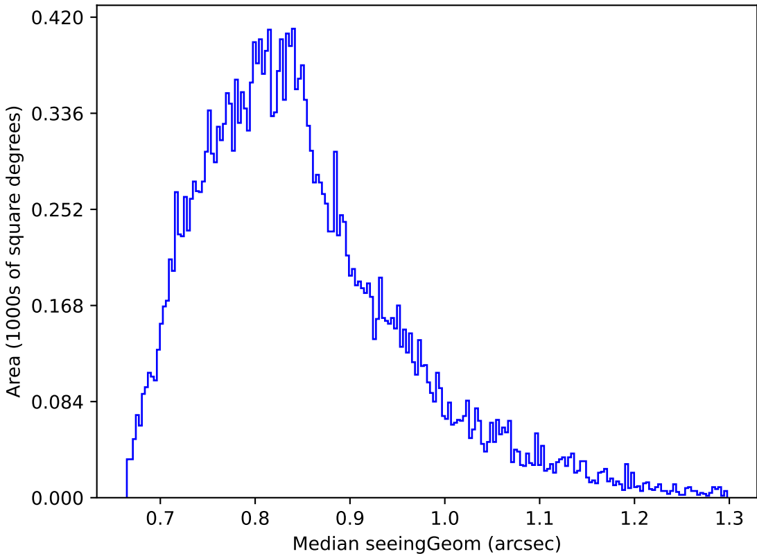
too_elab_r8_d3_giz_v3.4_10yrs Yr 1 z band: Median seeingGeom
