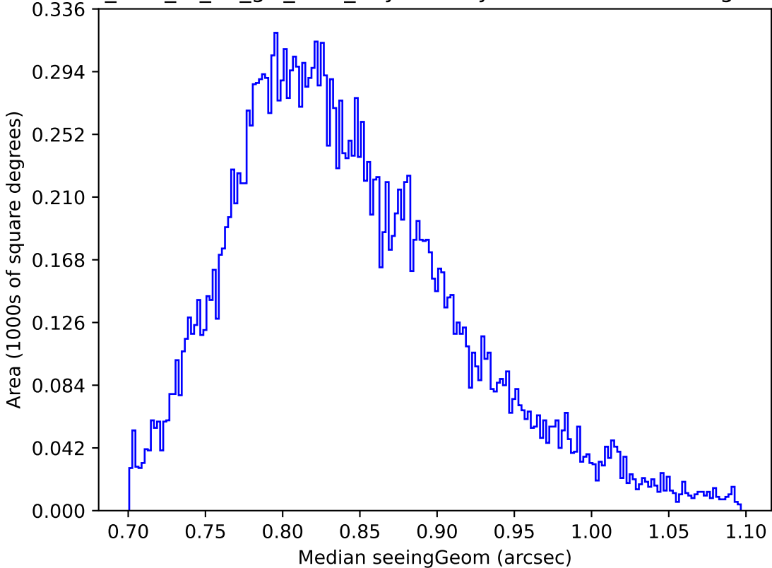
too_elab_r8_d3_giz_v3.4_10yrs Yr 1 y band: Median seeingGeom
