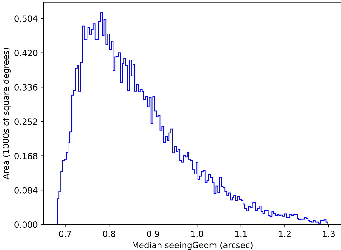
too_elab_r8_d3_giz_v3.4_10yrs Yr 1 r band: Median seeingGeom
