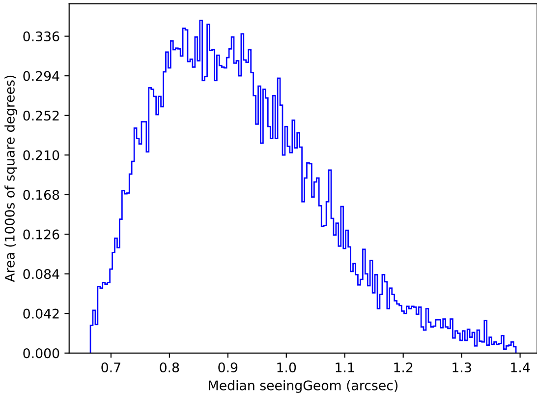
too_elab_r8_d3_giz_v3.4_10yrs Yr 1 g band: Median seeingGeom
