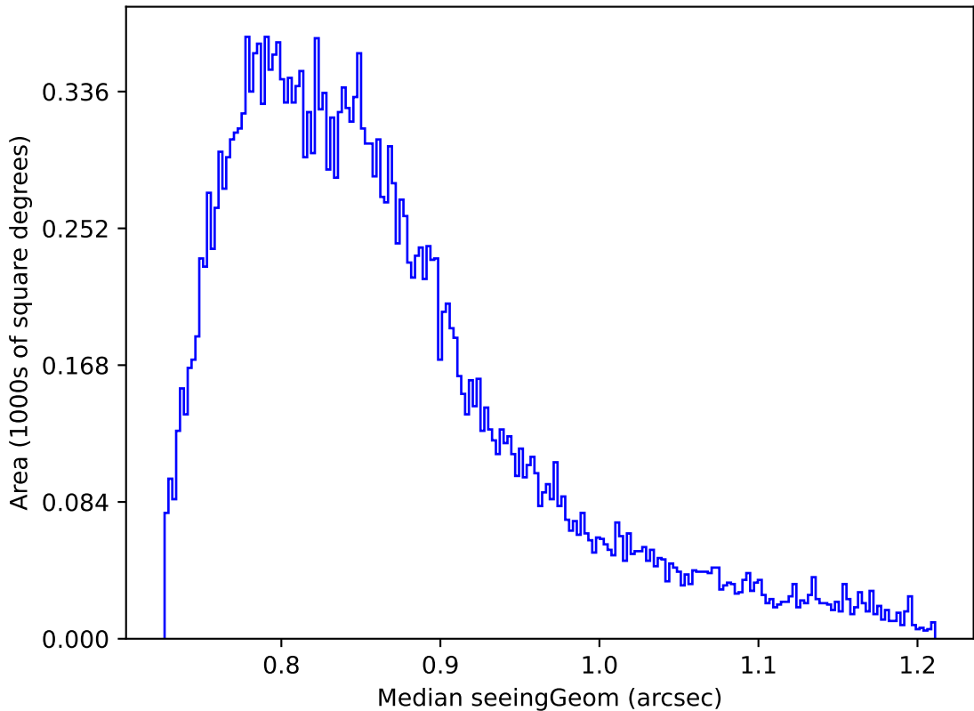
too_elab_r8_d3_giz_v3.4_10yrs Yr 1 all bands: Median seeingGeom
