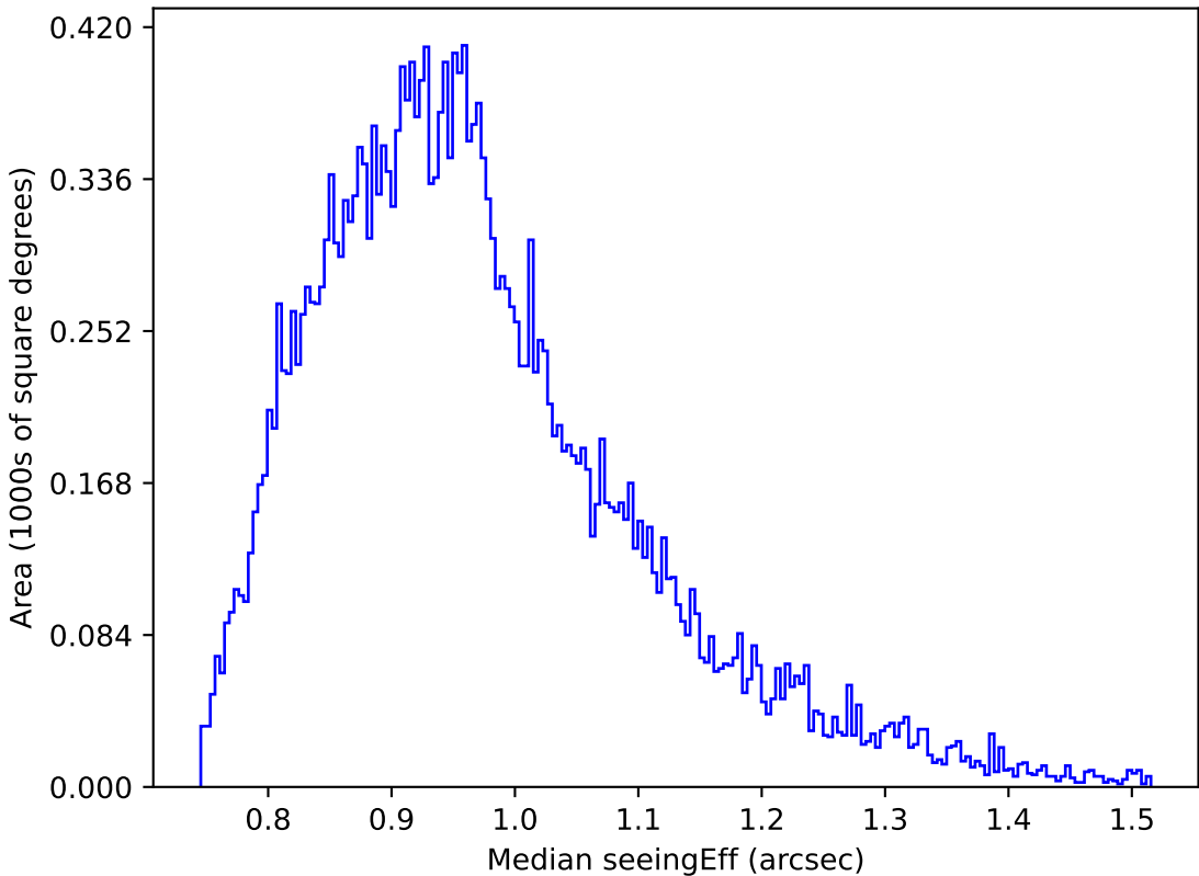
too_elab_r8_d3_giz_v3.4_10yrs Yr 1 z band: Median seeingEff
