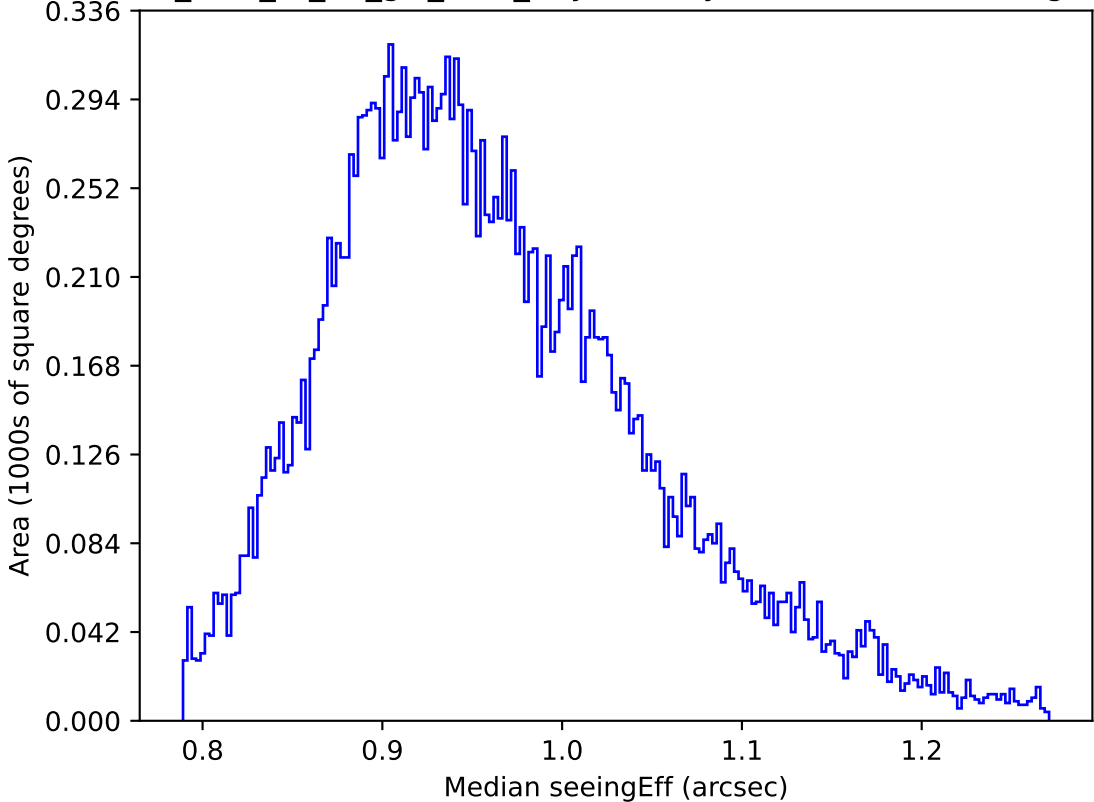
too_elab_r8_d3_giz_v3.4_10yrs Yr 1 y band: Median seeingEff
