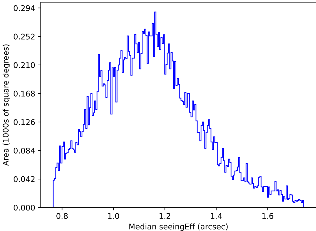
too_elab_r8_d3_giz_v3.4_10yrs Yr 1 u band: Median seeingEff
