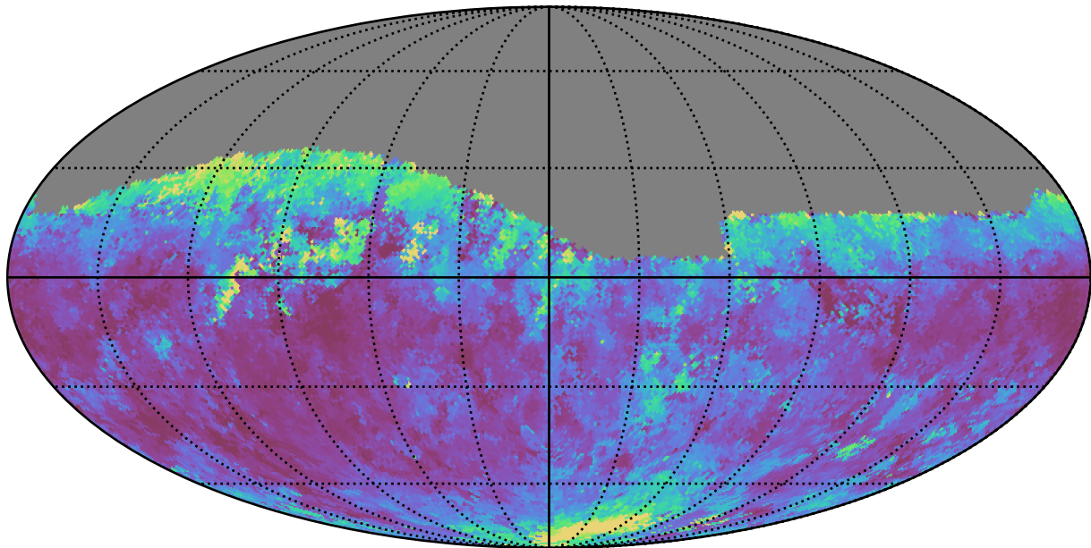
too_elab_r8_d3_giz_v3.4_10yrs Yr 1 r band: Median seeingEff
