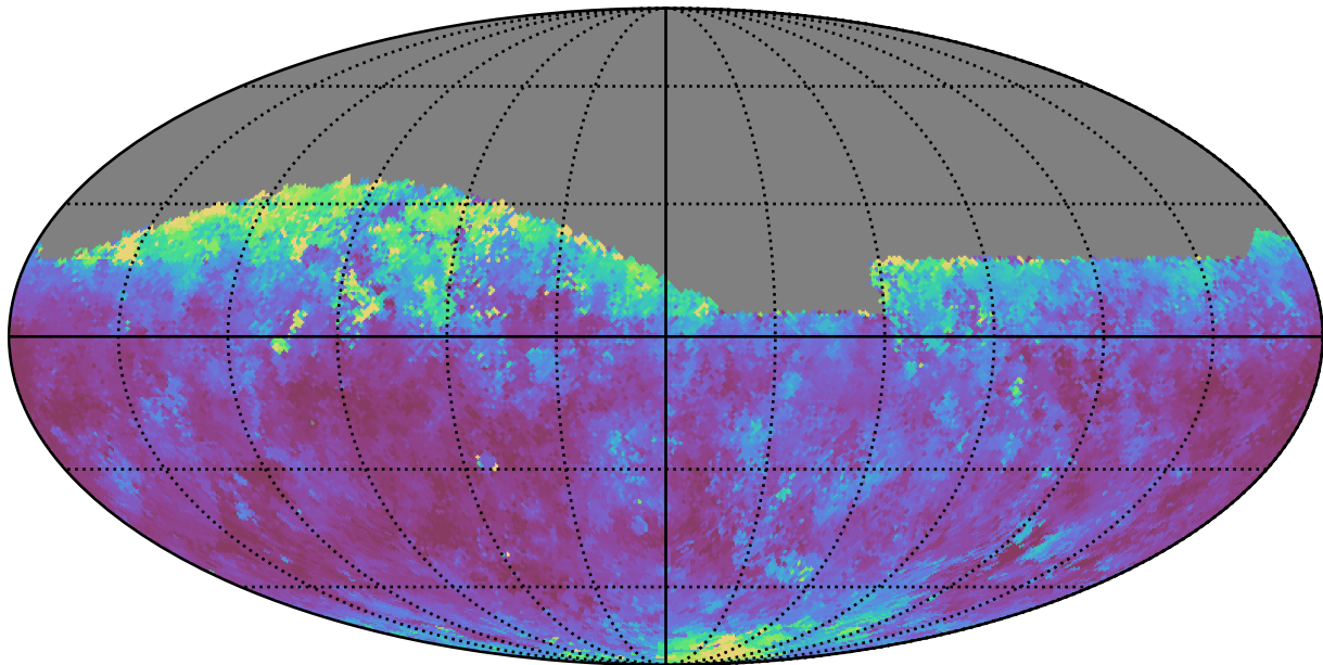
too_elab_r8_d3_giz_v3.4_10yrs Yr 1 i band: Median seeingEff
