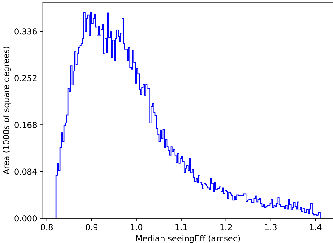
too_elab_r8_d3_giz_v3.4_10yrs Yr 1 all bands: Median seeingEff
