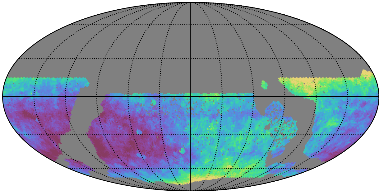
too_elab_r8_d3_giz_v3.4_10yrs WFD z band: Median seeingEff
