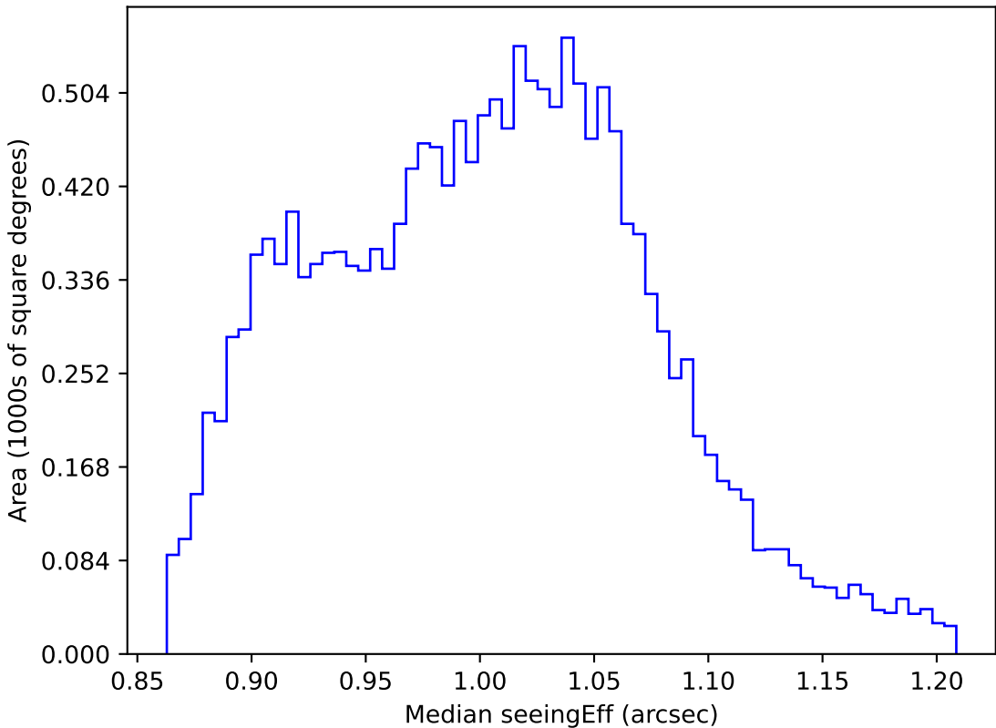
too_elab_r8_d3_giz_v3.4_10yrs WFD z band: Median seeingEff
