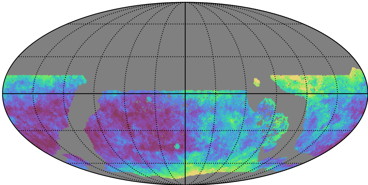
too_elab_r8_d3_giz_v3.4_10yrs WFD y band: Median seeingEff
