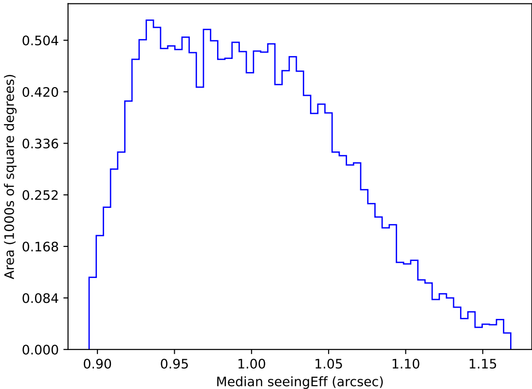
too_elab_r8_d3_giz_v3.4_10yrs WFD y band: Median seeingEff
