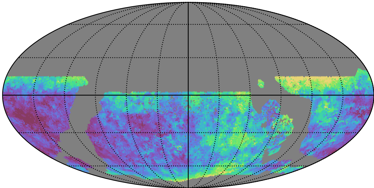
too_elab_r8_d3_giz_v3.4_10yrs WFD u band: Median seeingEff
