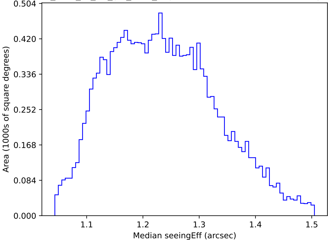
too_elab_r8_d3_giz_v3.4_10yrs WFD u band: Median seeingEff
