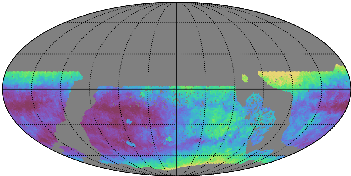
too_elab_r8_d3_giz_v3.4_10yrs WFD r band: Median seeingEff
