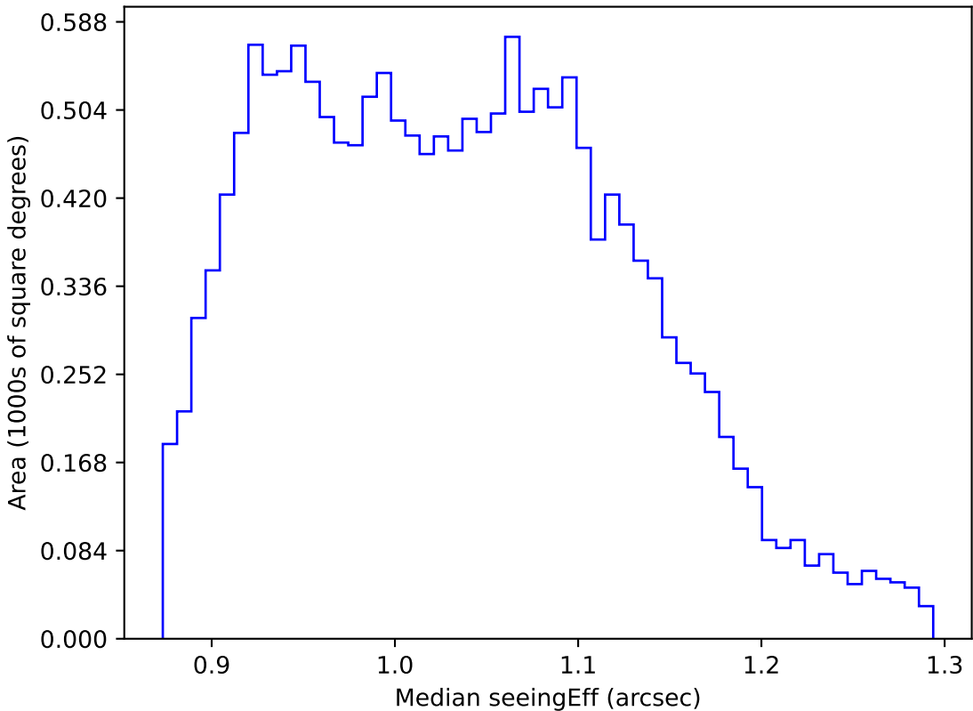
too_elab_r8_d3_giz_v3.4_10yrs WFD r band: Median seeingEff
