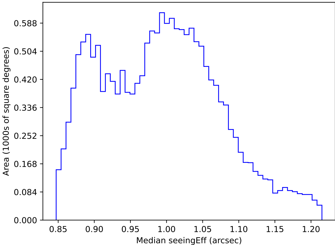
too_elab_r8_d3_giz_v3.4_10yrs WFD i band: Median seeingEff
