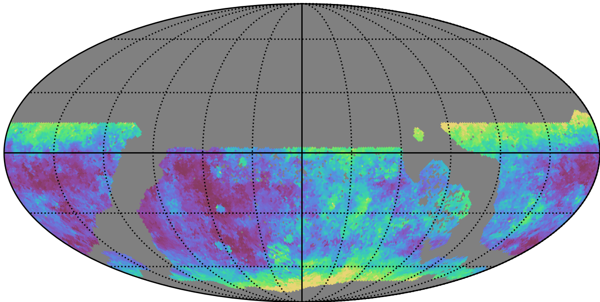
too_elab_r8_d3_giz_v3.4_10yrs WFD g band: Median seeingEff
