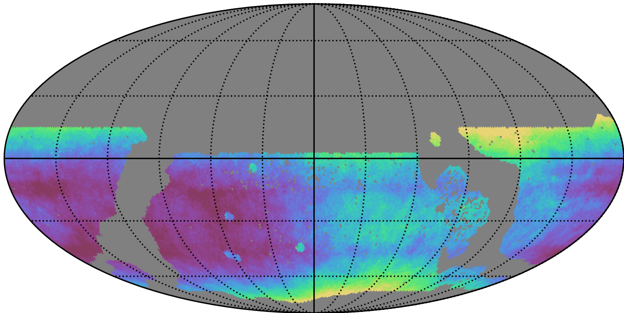
too_elab_r8_d3_giz_v3.4_10yrs WFD all bands: Median seeingEff
