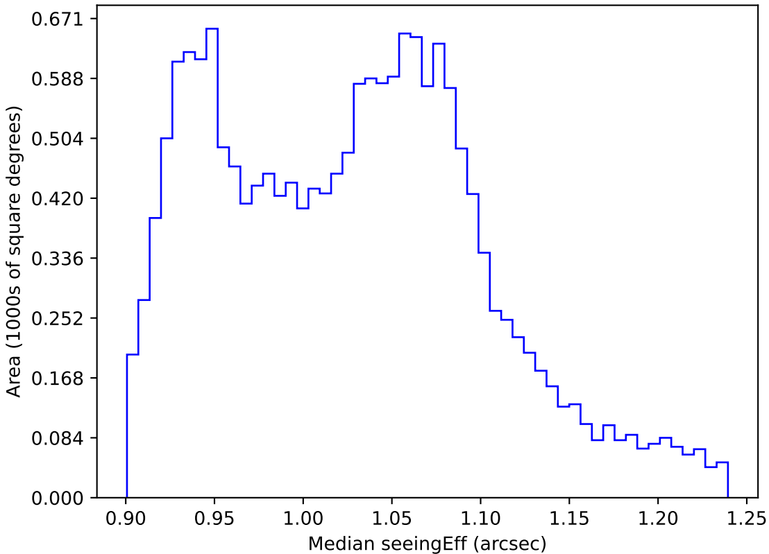
too_elab_r8_d3_giz_v3.4_10yrs WFD all bands: Median seeingEff
