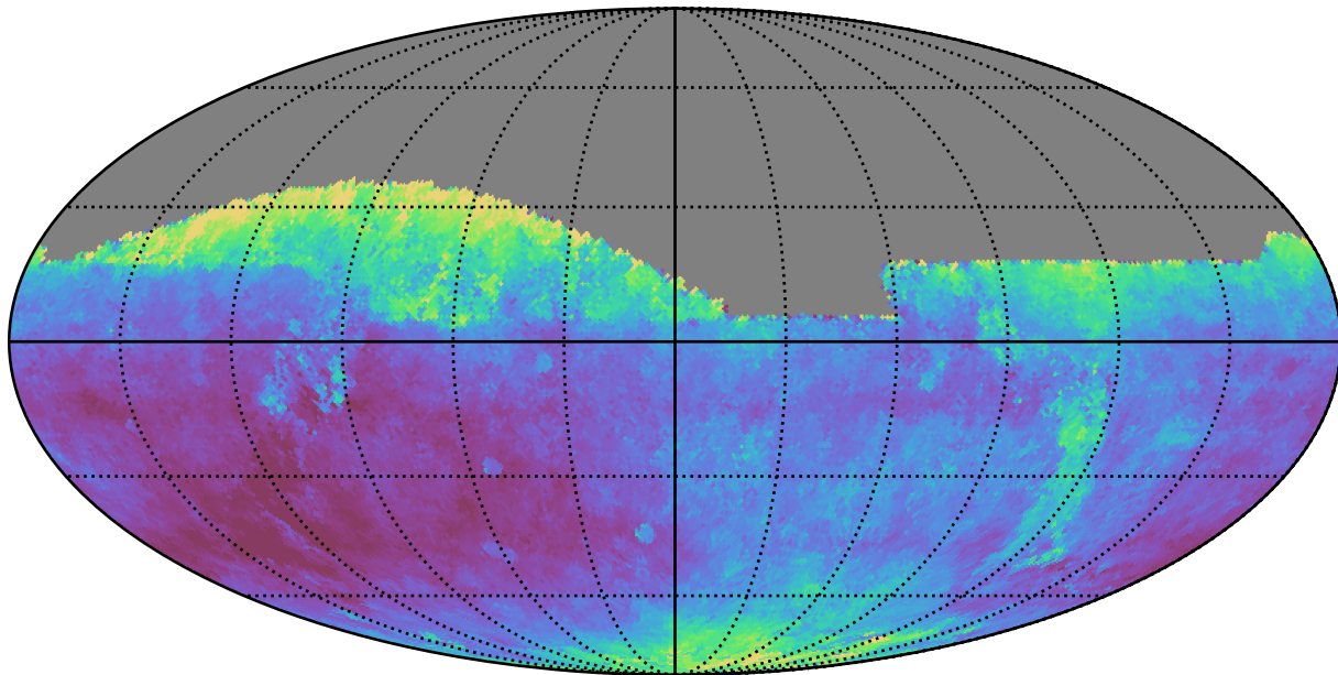
too_elab_r8_d3_giz_v3.4_10yrs All sky z band: Median seeingEff
