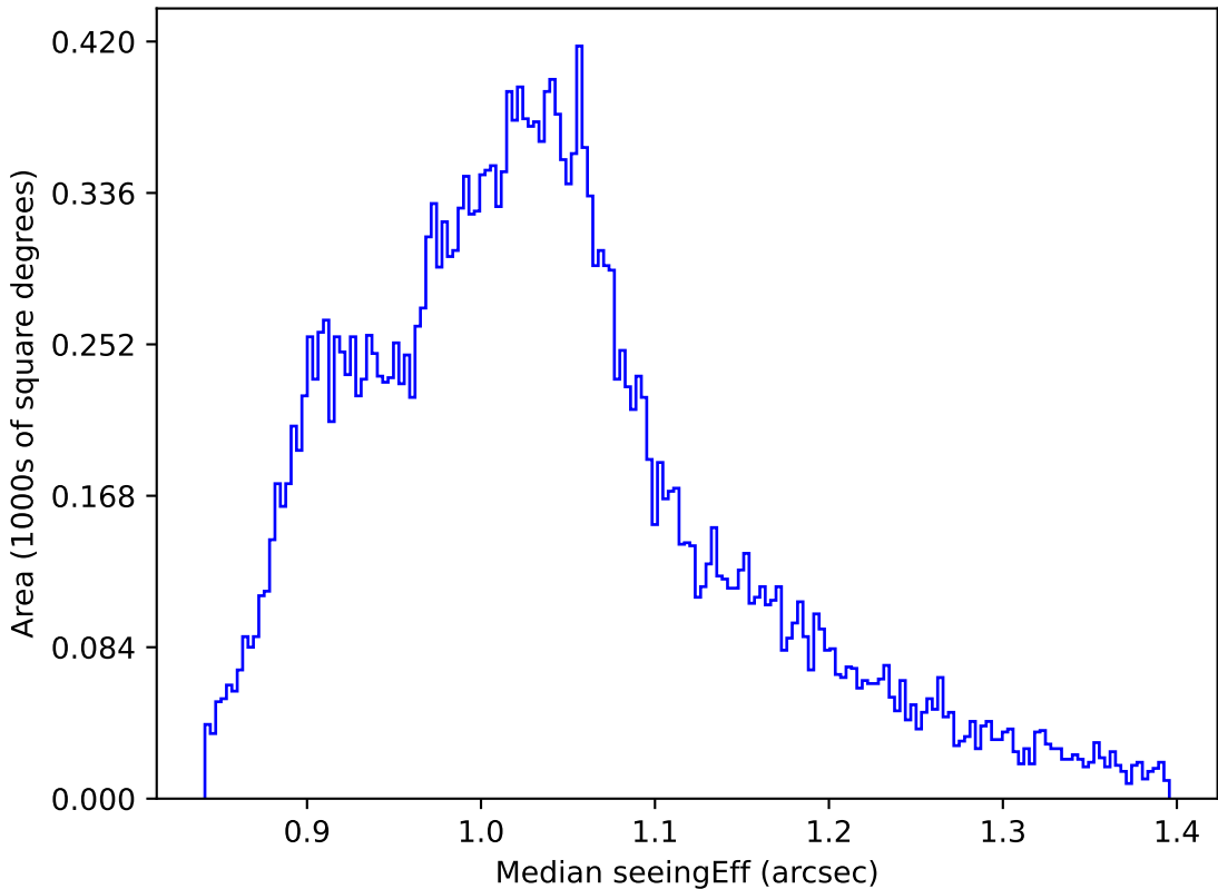
too_elab_r8_d3_giz_v3.4_10yrs All sky z band: Median seeingEff
