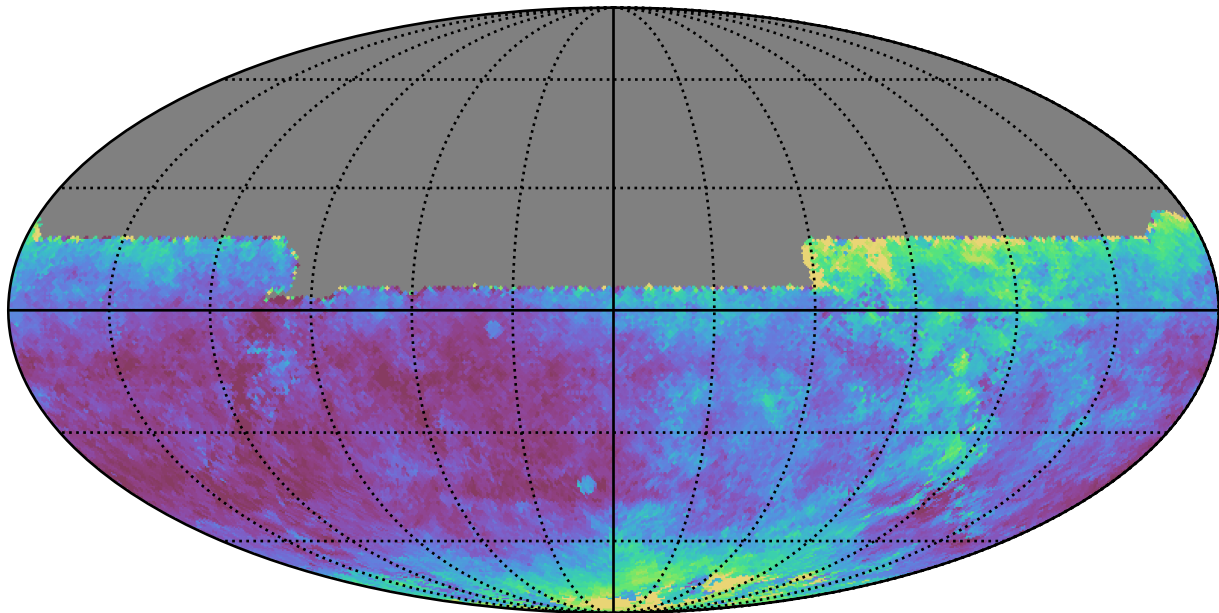
too_elab_r8_d3_giz_v3.4_10yrs All sky y band: Median seeingEff
