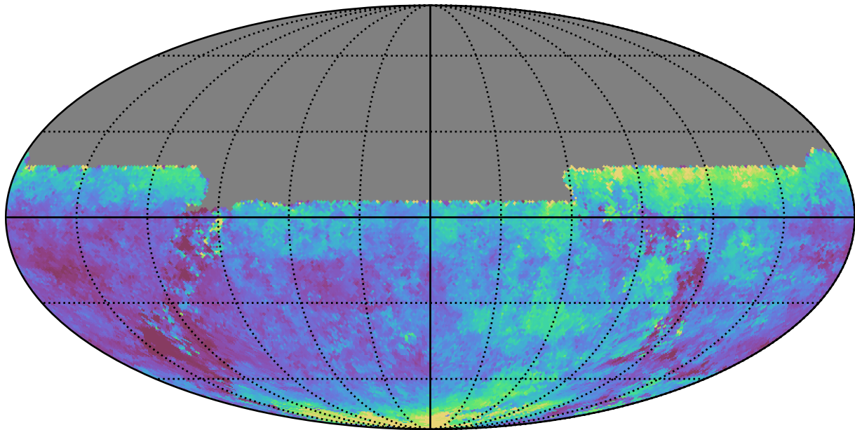
too_elab_r8_d3_giz_v3.4_10yrs All sky u band: Median seeingEff
