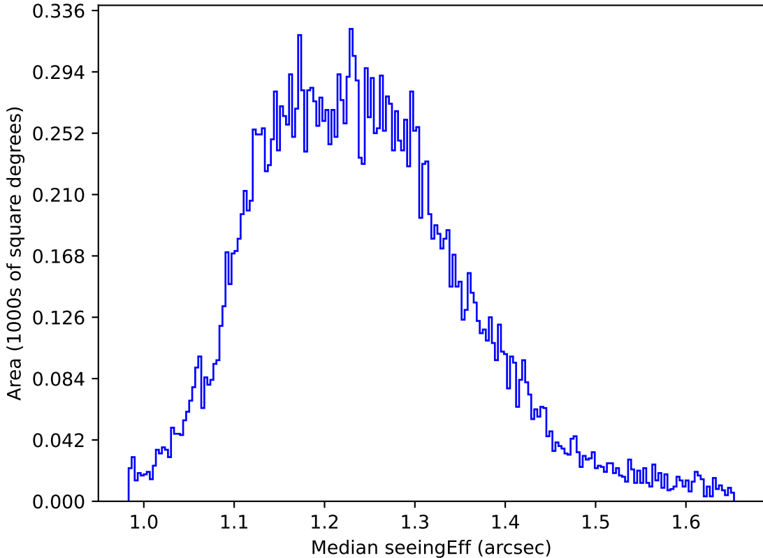
too_elab_r8_d3_giz_v3.4_10yrs All sky u band: Median seeingEff
