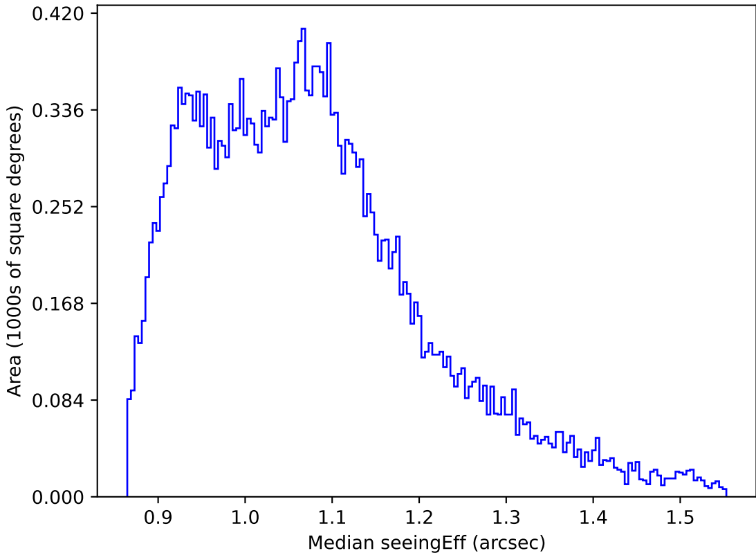
too_elab_r8_d3_giz_v3.4_10yrs All sky r band: Median seeingEff
