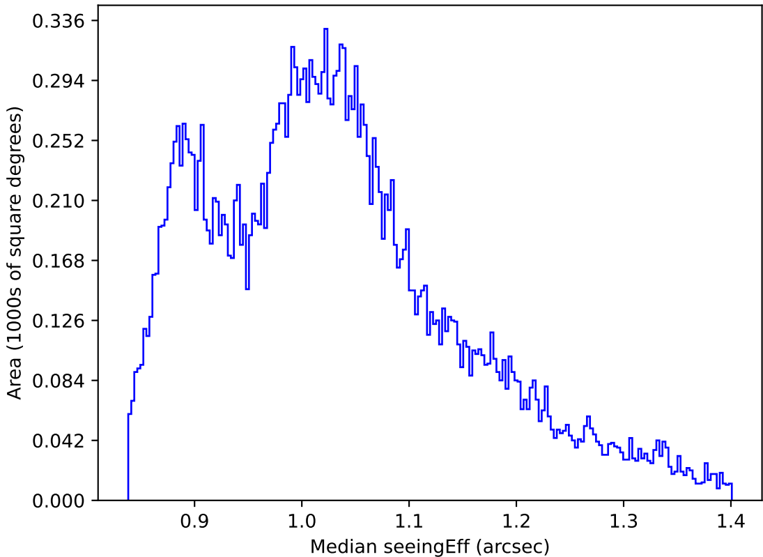
too_elab_r8_d3_giz_v3.4_10yrs All sky i band: Median seeingEff
