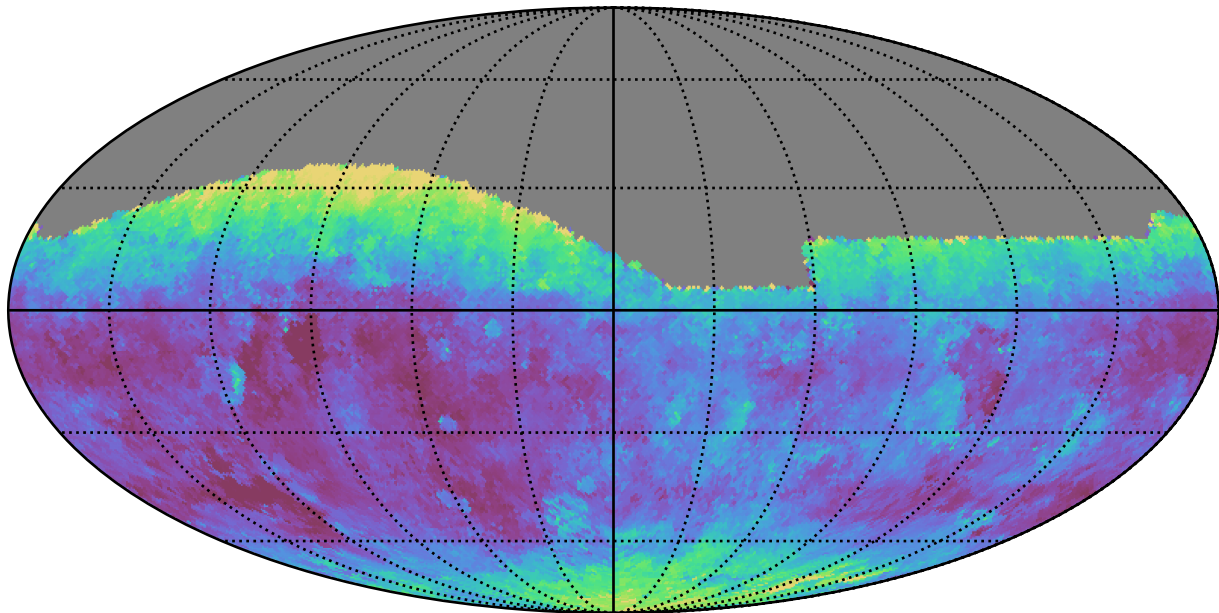
too_elab_r8_d3_giz_v3.4_10yrs All sky g band: Median seeingEff
